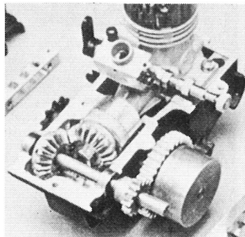
Latest Graupner importation trials motorbike complete with knobbles — available in electric power or with i.c., clever gearbox for same shown on right.
